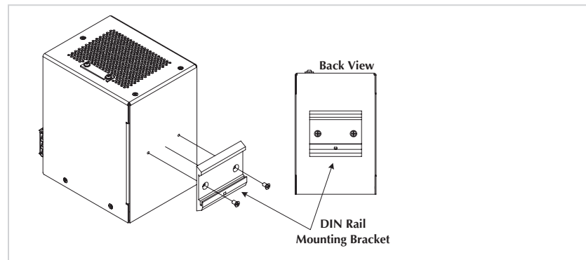
Figure 8: DIN-Rail Bracket
